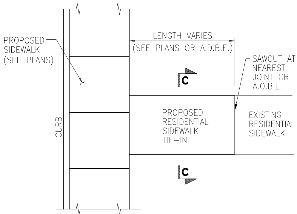
SIDEWALK TIE-IN WITH RESIDENTIAL WALK
